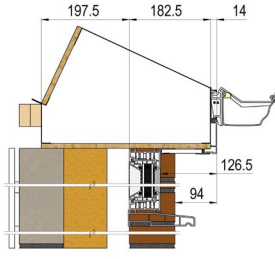
Brick & Block
