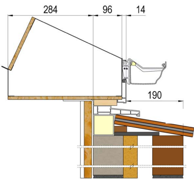
-190mm soffit
