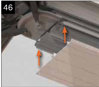
Moving inside the roof, fit the ridge undercladding to the ridge.
