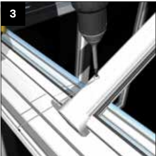
3 Secure the upper Cornice section using the wire ties at each glazing bar. Hook the wire tie into the pre-drilled hole in the upper Cornice section and screw fix into the glazing bar, ensuring the upper section remains parallel to the frames/roof line.
