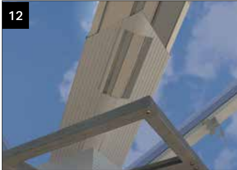
Fit the valley plate CHA016 (refer to steps 1-5, valley standard classic).
