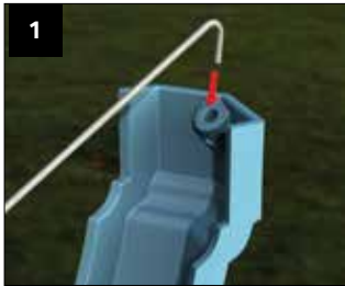
1 Prior to fitting the corner insert the special longer wire tie CRN012, into the corner as indicated
