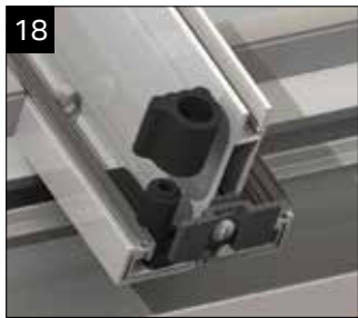
18 Snap off a gromet from the kit, this will slot over the upstand on the glazing stop. Repeat steps 35 & 36 for all glazing bars on the roof.
