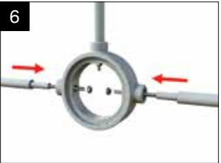
Insert threaded bar into the ring, and again finger tighten the nyloc nuts.
