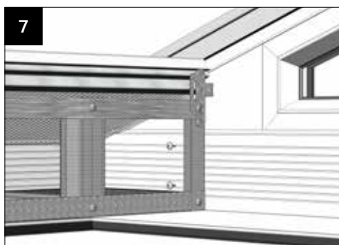
7 Fix the vertical frame into the fascia board using 2x CHAA006 (M4 x 13mm) self drill Phillips, wafer head screws (supplied).
