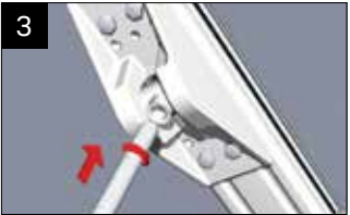
Measure, cut and attach the horizontal threaded bars (ensure sufficient engagement of the bar into the brackets) – it is essential that the tie bar boss is central. Take the boss ring, and loosely assemble the threaded bars to check they terminate inside the ring. Dis-assemble.
