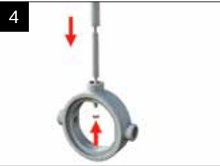
Insert the smaller diameter pieces of PVCu conduit inside. Offer into the boss ring and finger tighten the nyloc nut.
