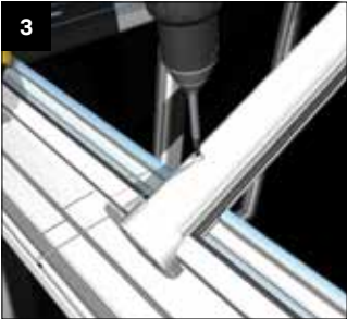
Secure the upper section using the wire ties at each glazing bar. Hook the wire tie into the pre-drilled hole in the upper section and screw fix into the glazing bar, ensuring the upper section remains parallel to the frames/roof line.
