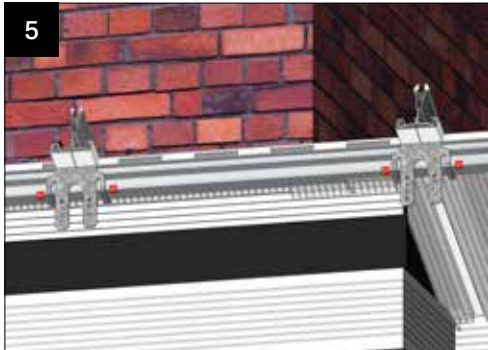
5 Fit the appropriate polycarbonate-LUVGS panels as shown in the main internal insulated pelmet installation guide (page 16) and bend the bracket legs to secure.
