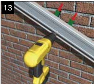
Drill the starter rafters/masonry within 200mm of the ridge and eaves plus at least one more equidistant hole between the two. Pack behind the starter bar and fix with an appropriate masonry anchor.
