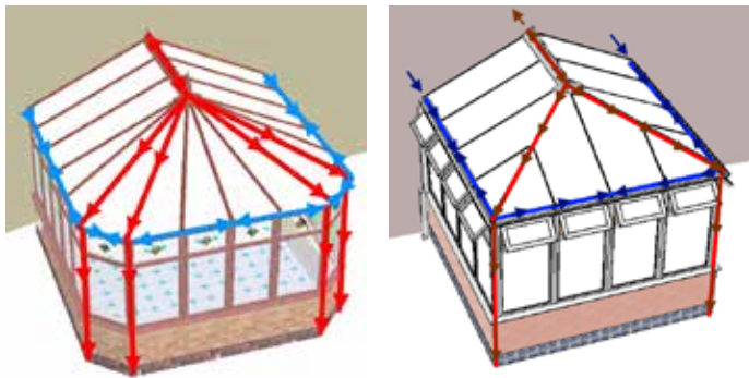
Diagram of the forces and load paths when a roof without a tie bar is loaded (downward load) - Compression in red, tension in blue.
