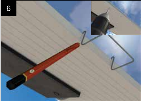
Fit the cloaking panel support clips CHA002 onto the valley cladding (2 per valley side supplied). Space out clips and temporarily hook over the valley cladding. Mark the leg positions then remove the clips. Drill a 5mm hole at each leg position as shown. NOTE: AVOID DRILLING THROUGH THE VALLEY DRIP PROFILE
