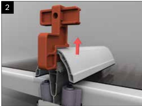
Lift the capping removal tool up, releasing the top cap legs from the aluminium.
