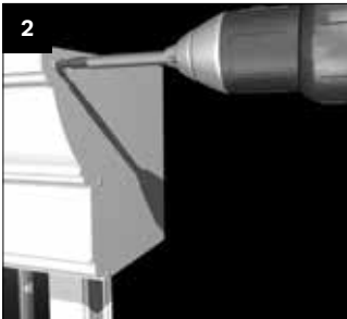
GUTTER STOP END DETAIL - Used with lean-to roofs, gable roofs or when then gutter returns along the host wall. Secure the end plate into position using the fixings provided (CRN008).
