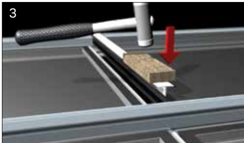
Now lift the sealed unit that goes on the lower slope into position, turn the upper profile over, place it into position and tap down the profile using a non marking plastic mallet. Wipe clean any sealant from the unit face. NOTE: WE RECOMMEND A SECOND PERSON TO SUPPORT THE MUNTIN FROM THE UNDERSIDE WHEN TAPPING DOWN.
