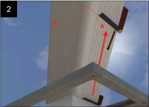
Using an angle finder (or joiners bevel). Draw a line on the valley cladding from the mark 'A' parallel to the eaves.
