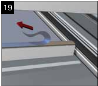
19 Tease the 'tail' of the glazing support trim tape free (ready to be pulled away when the sealed unit is finally in position).
