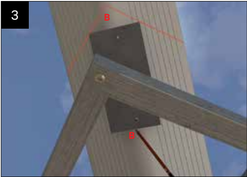
Temporarily position the valley fixing plate central of the valley with the top edges touching the marked lines. Mark either side of the plate (shown as 'B' on the cladding). Now remove valley fixing plate.
