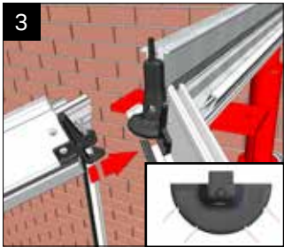
Fit hip bars by pushing the Spider arm hook over the Spider (aligning with outer marked notched positions) and then lowering onto the bolts in the eaves corners.
