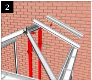
Fit and secure starter bars and side transoms to either side of the ridge. Locate on the bolts in both the eaves and ridge. Follow location plan for rafter position.
