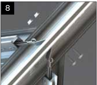
If two jack rafters are aligned either side of the hip, an M6 x 25mm bolt is used through both brackets and the pre-drilled holes in the hip. Secure with the provided flanged nuts.
