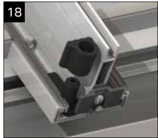
18 Snap off a gromet from the kit, this will slot over the upstand on the glazing stop. Repeat steps 35 & 36 for all glazing bars on the roof.
