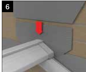
Offer up the horizontal flashing which should typically sit two courses above the stepped flashing. Trim to suit the roof pitch.
