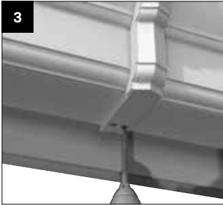
Whilst ensuring that the inline bracket remains located in position, screw fix using self drilling screws CRN007.
