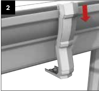
Offer up the CRN180 straight jointer, hook over the front lip of the gutter cover.
