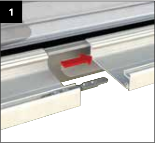
Attach the cleat CRN001 using 2 x CRN006 provided, on each side of the joint. Repeat for each of the 'layers'.
