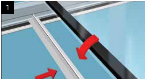
IF YOUR SEALED UNITS HAVE BEEN SUPPLIED WITH TAPED EDGES, ALWAYS REMOVE THE TAPE PRIOR TO INSTALLATION. Take the muntin bar profile (top and bottom section) that matches its corresponding sealed unit. Take the lower section and allow it to span between the two adjacent glazing bars. Lower into position the up slope sealed unit. NOTE: MUNTIN SHOULD BE SAME WIDTH AS UNIT.
