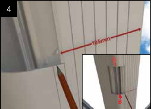
Then measure 105mm in from each side of the valley cladding and extend mark B top and bottom to form pencil rectangle. Cut out valley cladding.
