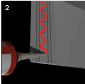
Trial fit the stepped flashing. Start installing from the gutter towards the ridge. Apply sealant (clear or grey low modulus neutral cure) along the two internal weather bar grooves.
